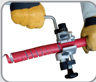
Stripping external sheath
