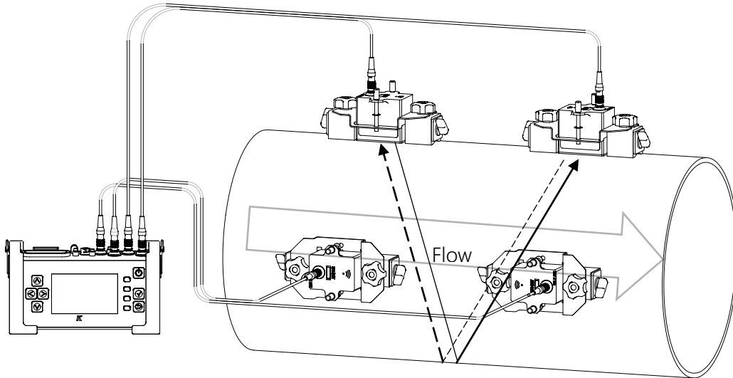
Flow / mass measurement configuration (1 or 2 path )
