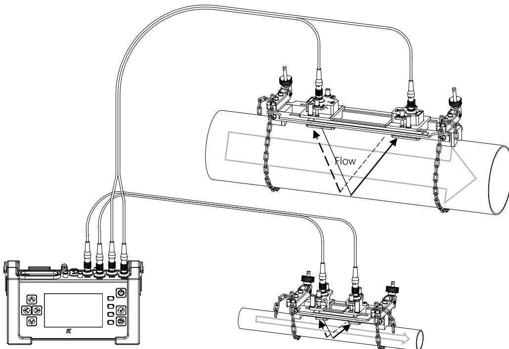
Flow / mass measurement configuration (two pipes at the same time )
